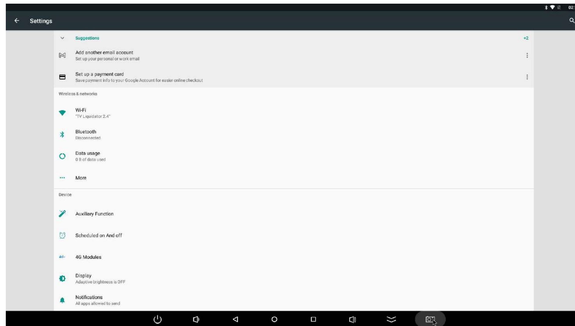
Settings Menu
