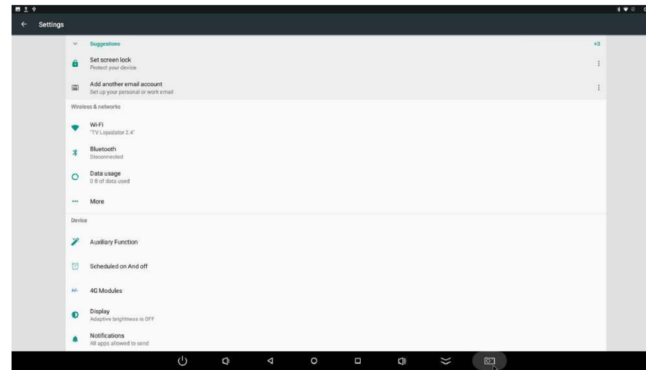
Settings Menu
